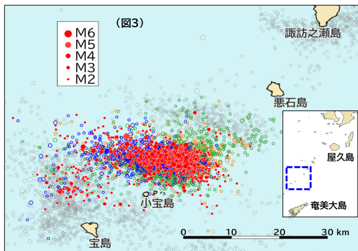
図3:震央分布図 1997/10/1 --- 2025/6/28 M ≥2.0 40km以浅 ●2025/6/21~6/28 ●2023/9/1~9/30 ●2021/12/1~12/31 ●2021/4/1~4/31 ○上記期間以外
